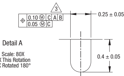
Figure 15. SKY16602-632LF Package Dimensions
